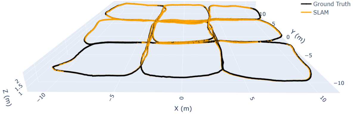
Figure 14: 3D trajectory plot, with ground truth trajectory shown in black and final estimated SLAM trajectory shown in orange.
