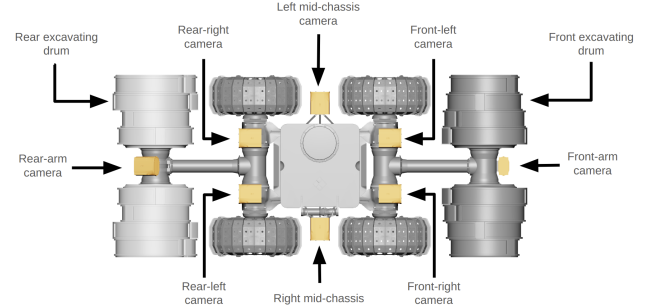
(b) Diagram of the the lunar robot showing the arrangement of its eight cameras.
