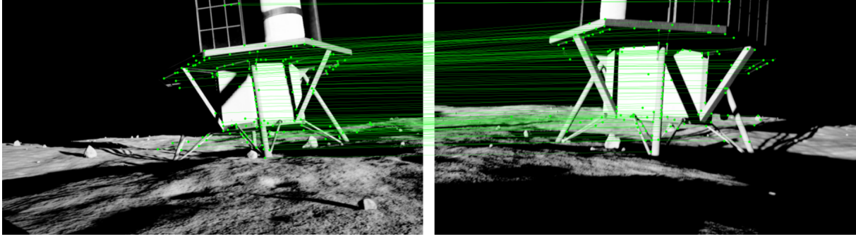
Figure 6: LightGlue feature matching on the lander between different viewpoints.
